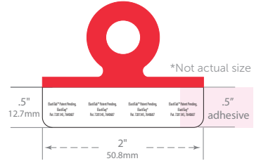
Die #2243 Recommended for items with a circumference of 1.59"–3.33" (40mm–84mm)
