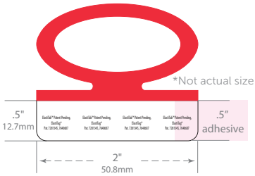
Die #2102 Recommended for items with a circumference of 4.4"–6.5" (111mm–165mm)
