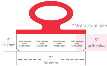
Die #2144 Recommended for items with a circumference of 2.7"–4.5" (68mm–114mm)
