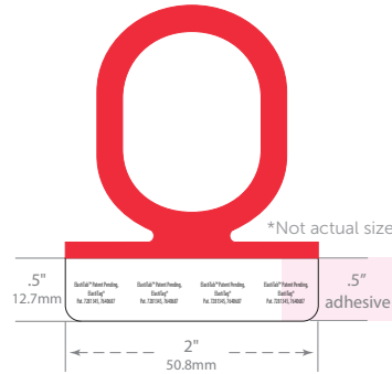
Die #2145 Recommended for items with a circumference of 4.5"–8.2" (114mm–208mm)
