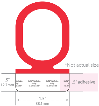
Die #2164 Recommended for items with a circumference of 4.5"–8.2" (114mm–208mm)
