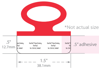
Die #2347 Recommended for items with a circumference of 2.7"–4.5" (68mm–114mm)
