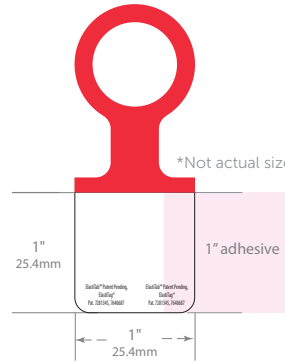
Die #2312 Recommended for items with a circumference of 2.6"–3.8" (66mm–97mm)
